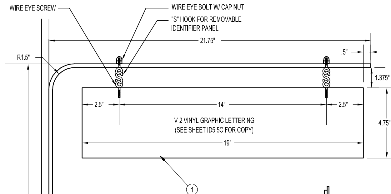
TOP VIEW SCALE 1/4" = 1"
